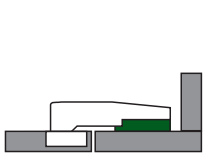
Cup hinge: steel, nickel-plated Hinge arm: Zamak, nickel-plated
