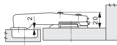
Drawing with mounting plate, height 02
