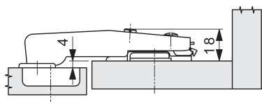
Drawing with mounting plate, height 00
