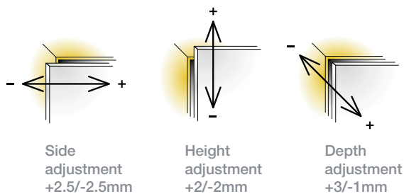
Door adjustment
