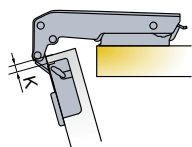
Drawing shows application on D=2mm mounting plate
